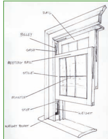
Figure 2. Double-hung window
