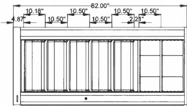
Elevation C
